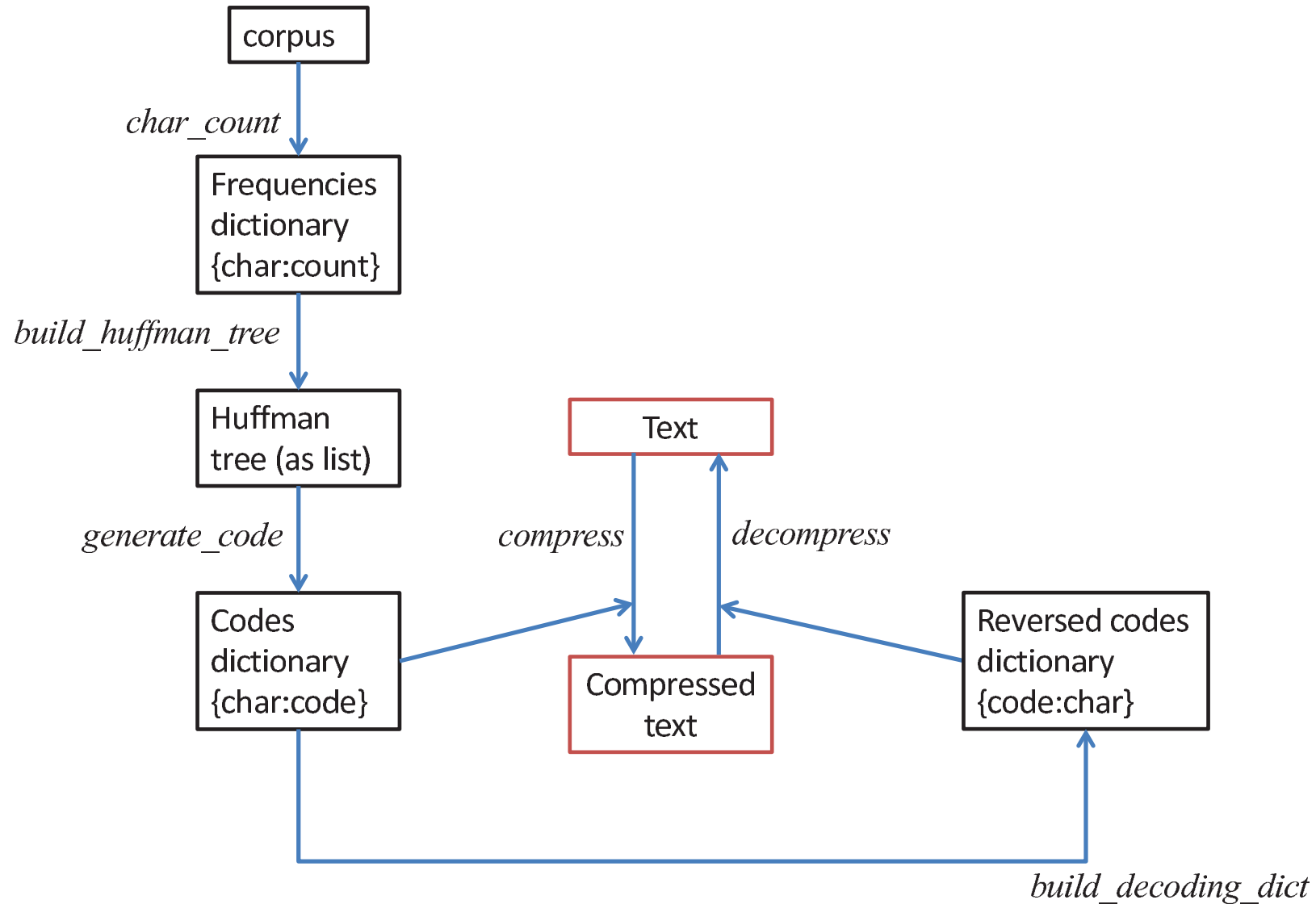
Flow diagram of Huffman compression process
